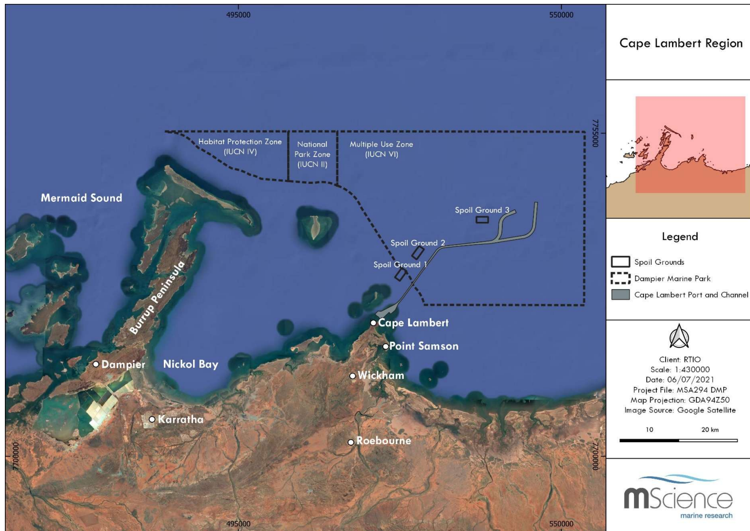
Figure 1-1 Cape Lambert region
