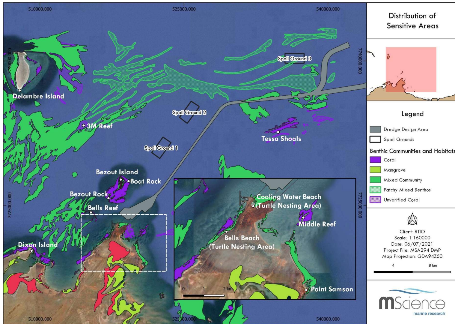
Figure 3-1 Distribution of sensitive areas around Cape Lambert
