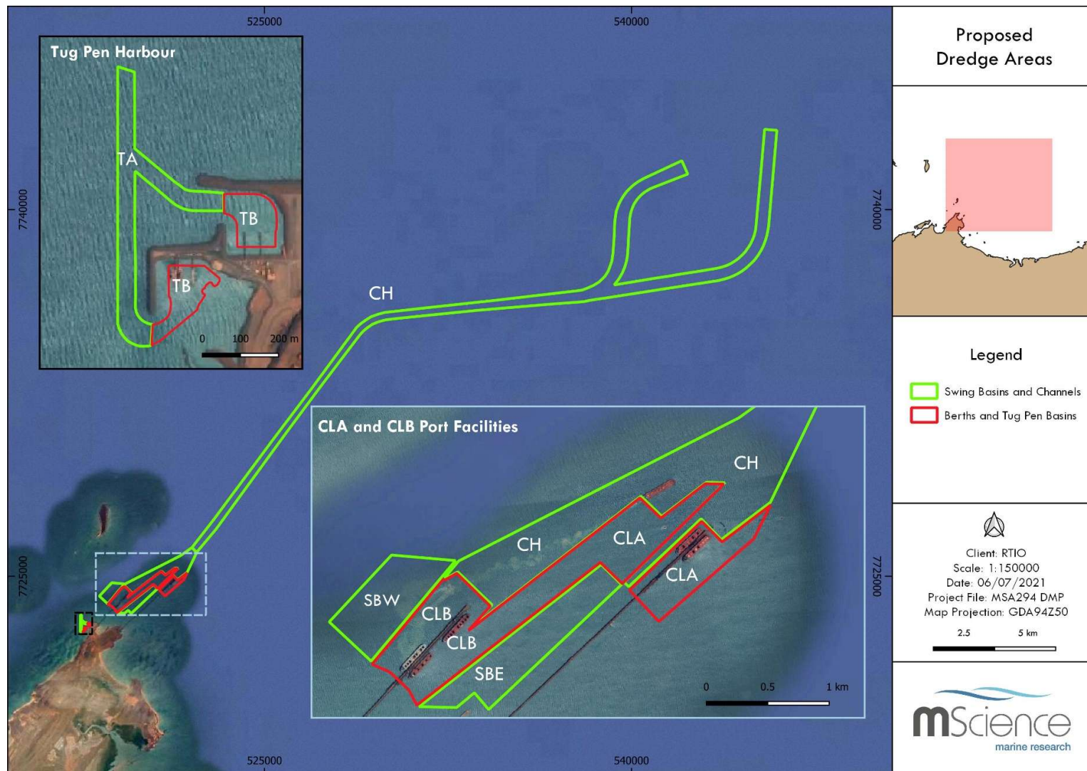
Figure 1-2 Proposed dredge areas
