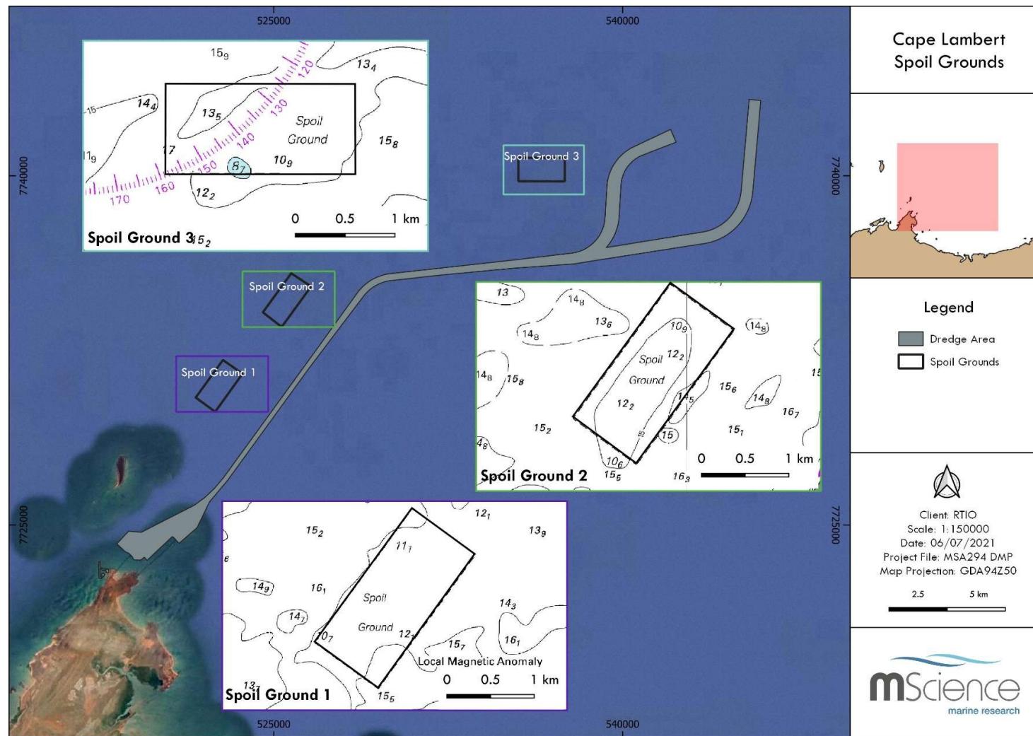
Figure 1-3 Spoil disposal sites
