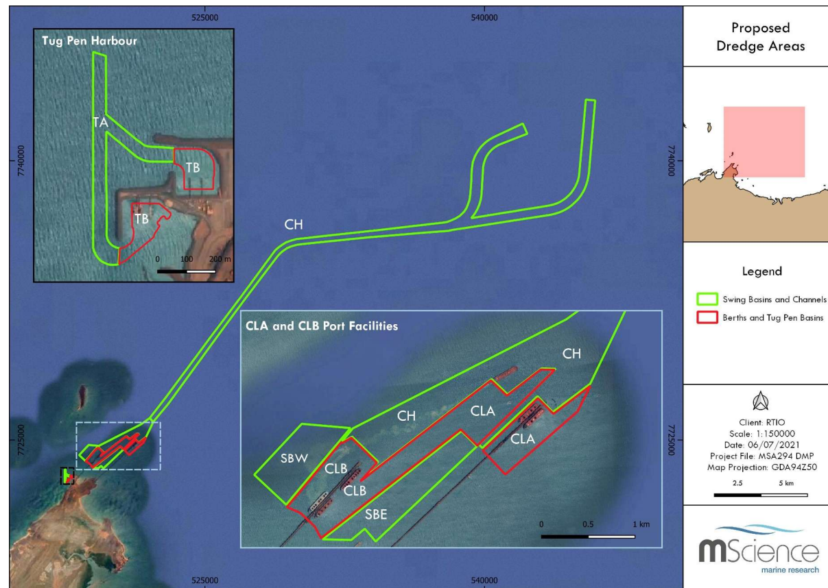
Figure 1-2 Proposed dredge areas
